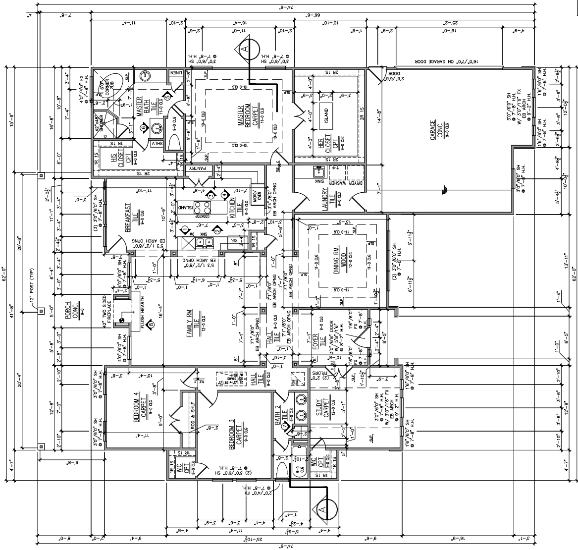
FLOOR PLAN
