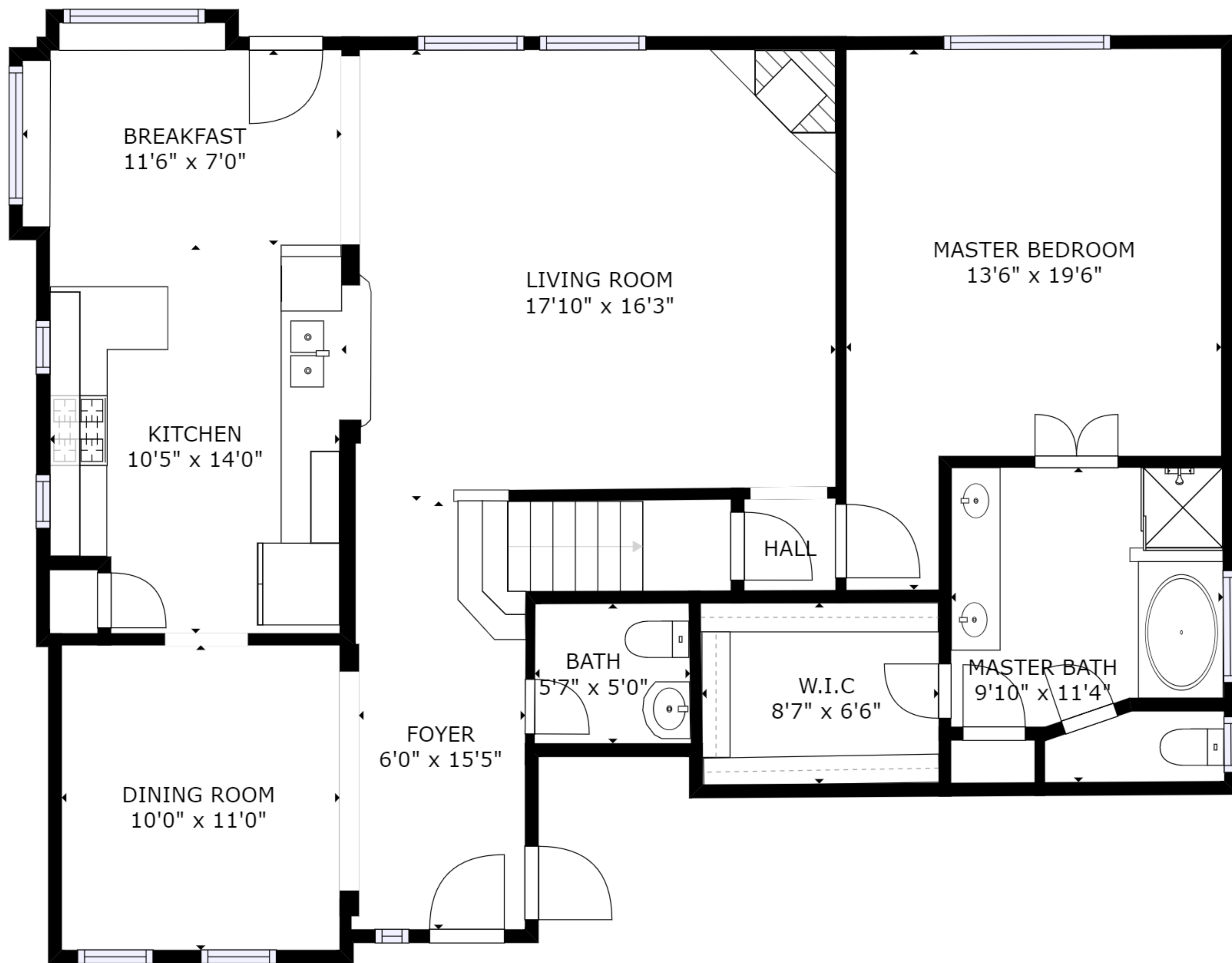
FLOOR 1
