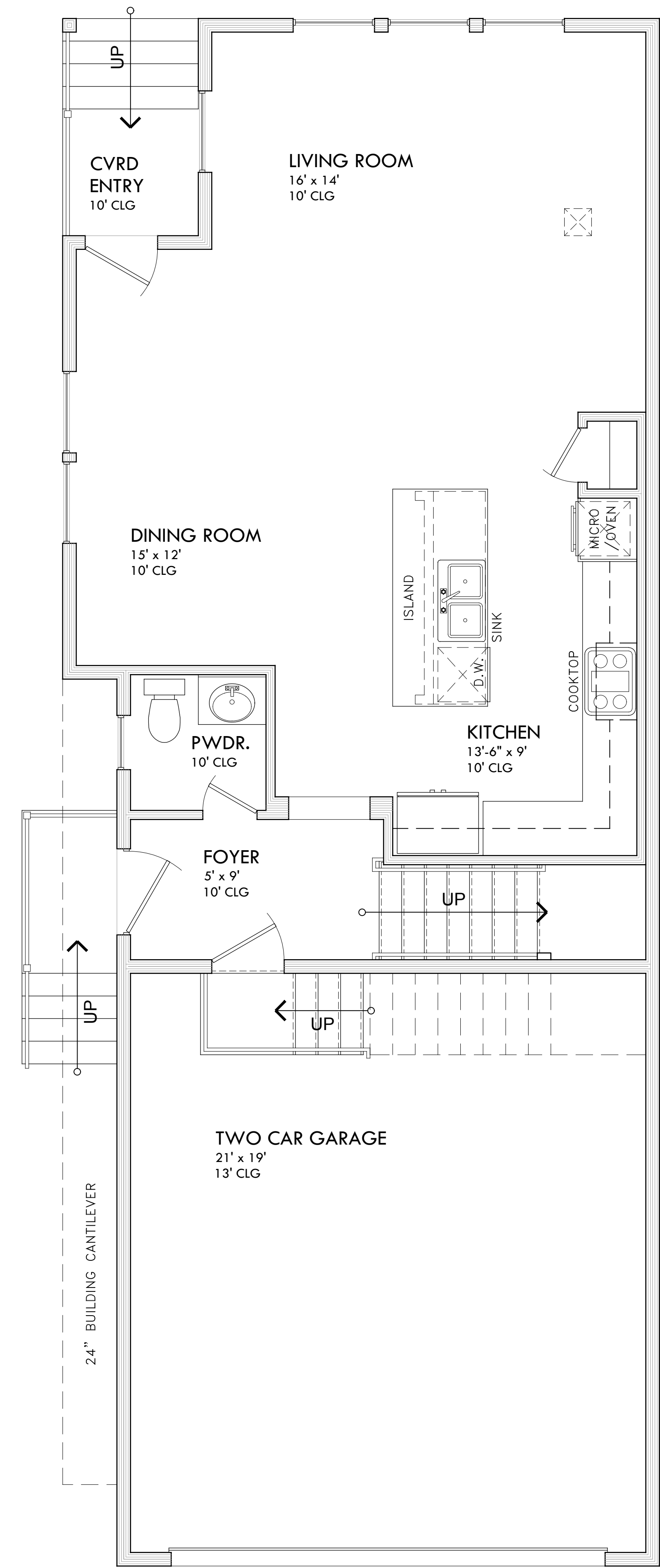
1st FLOOR PLAN
