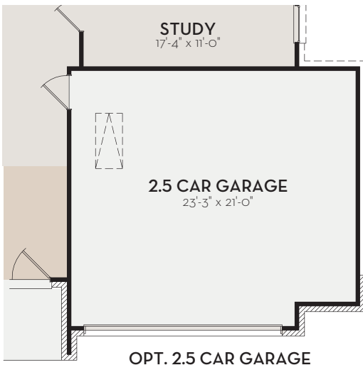
OPT. 2.5 CAR GARAGE
