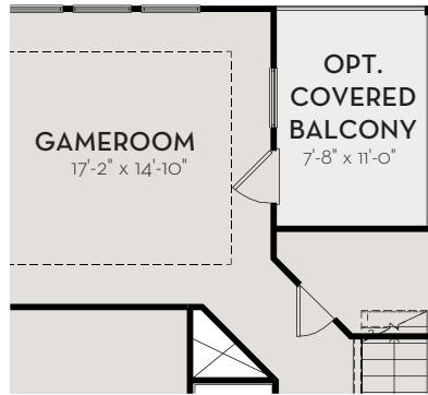
OPT. COVERED BALCONY NOT AVAILALE W/ COVERED PATIO
