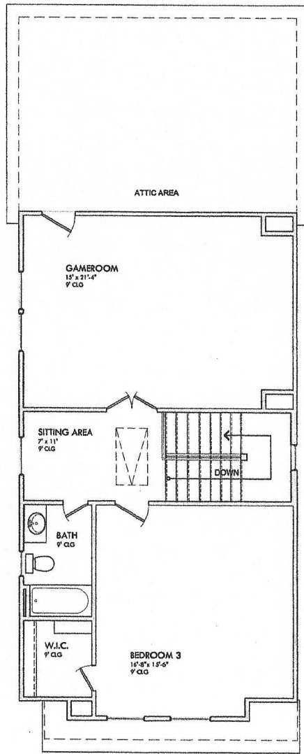
3rd FLOOR PLAN
