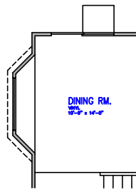
OPTIONAL WINDOW SEAT AT DINING
