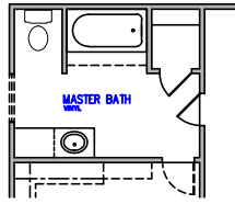
OPTIONAL LINEN AT MASTER BEDROOM
