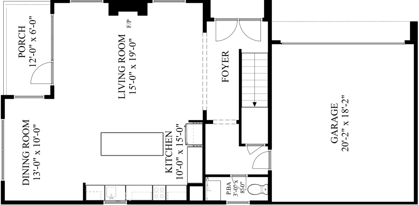
FIRST FLOOR
