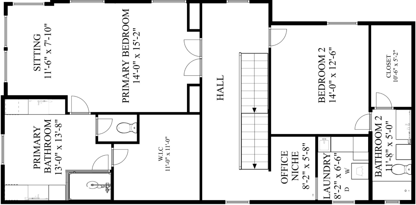
SECOND FLOOR
