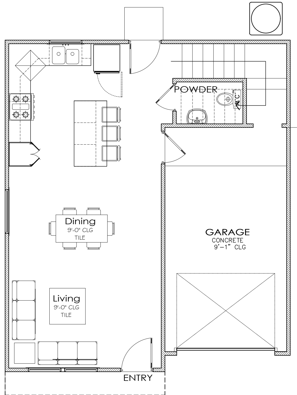
1 FLOOR PLAN FIRST FLOOR
