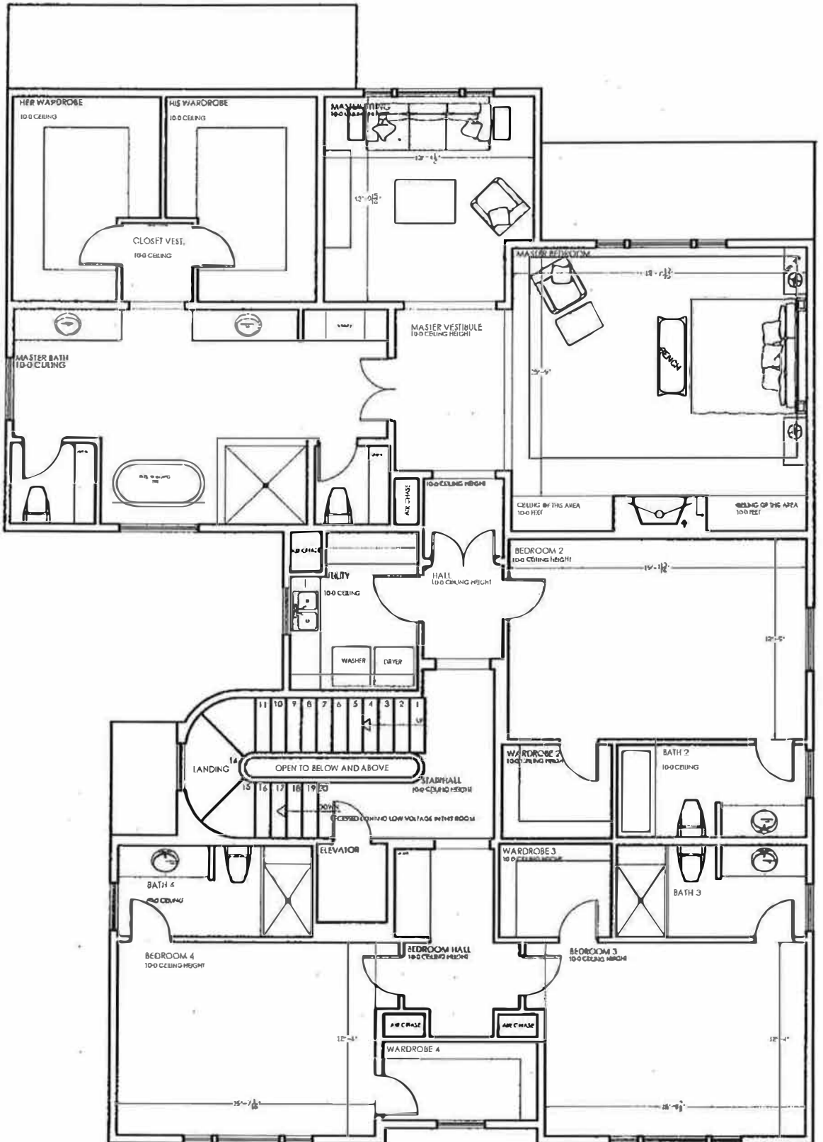
2109 DICKEY PLACE SECOND FLOOR
