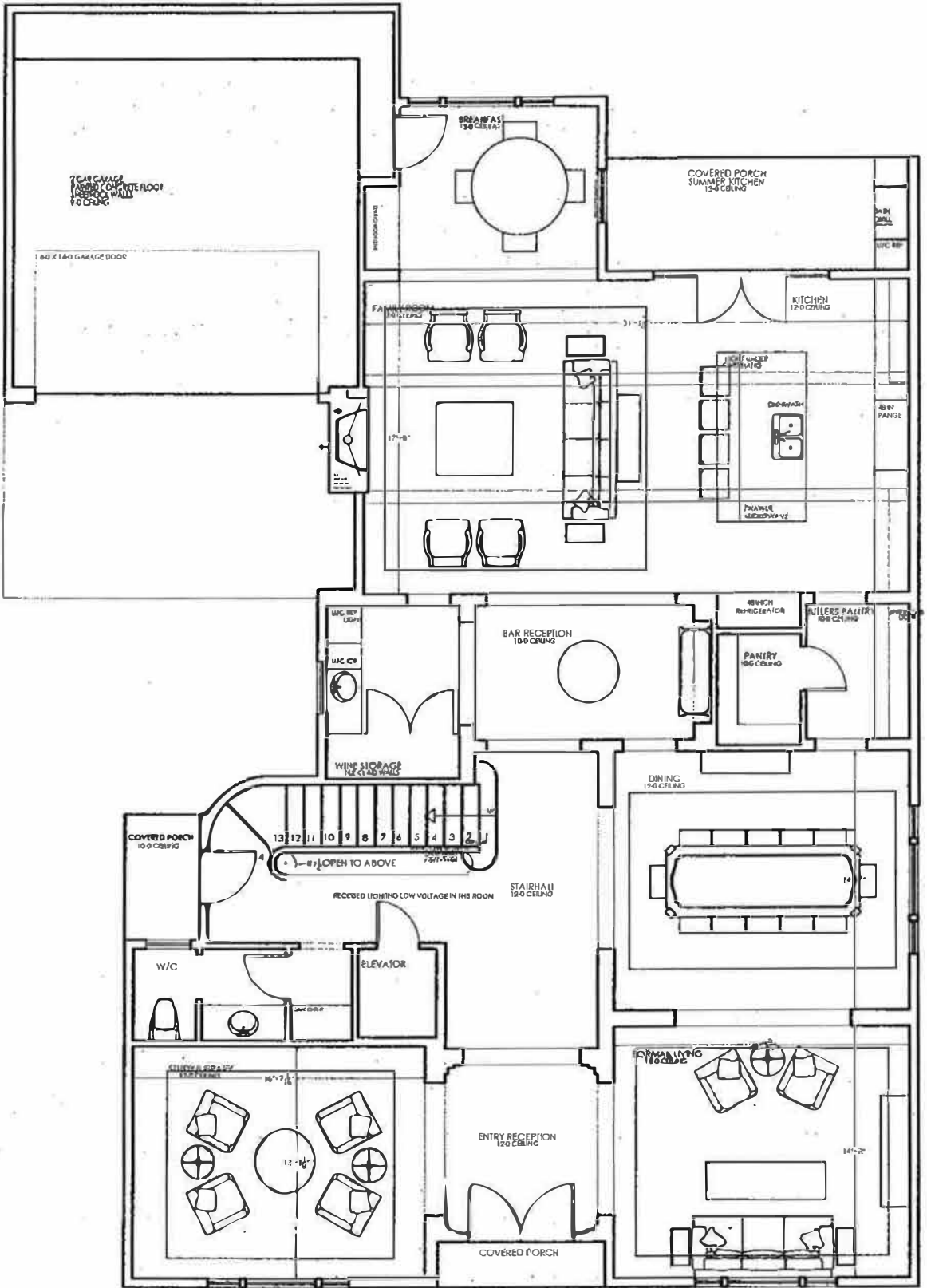
2109 DICKEY PLACE FIRST FLOOR
