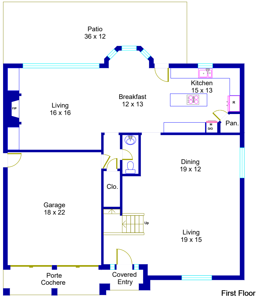
First Floor
