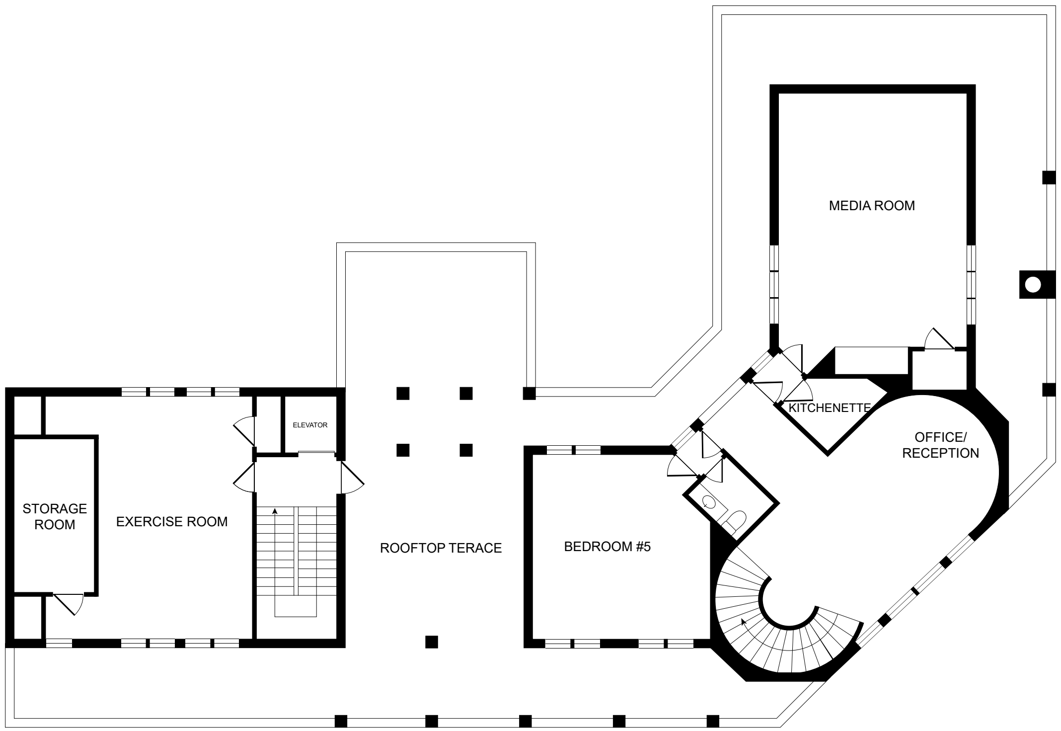
3RD FLOOR
