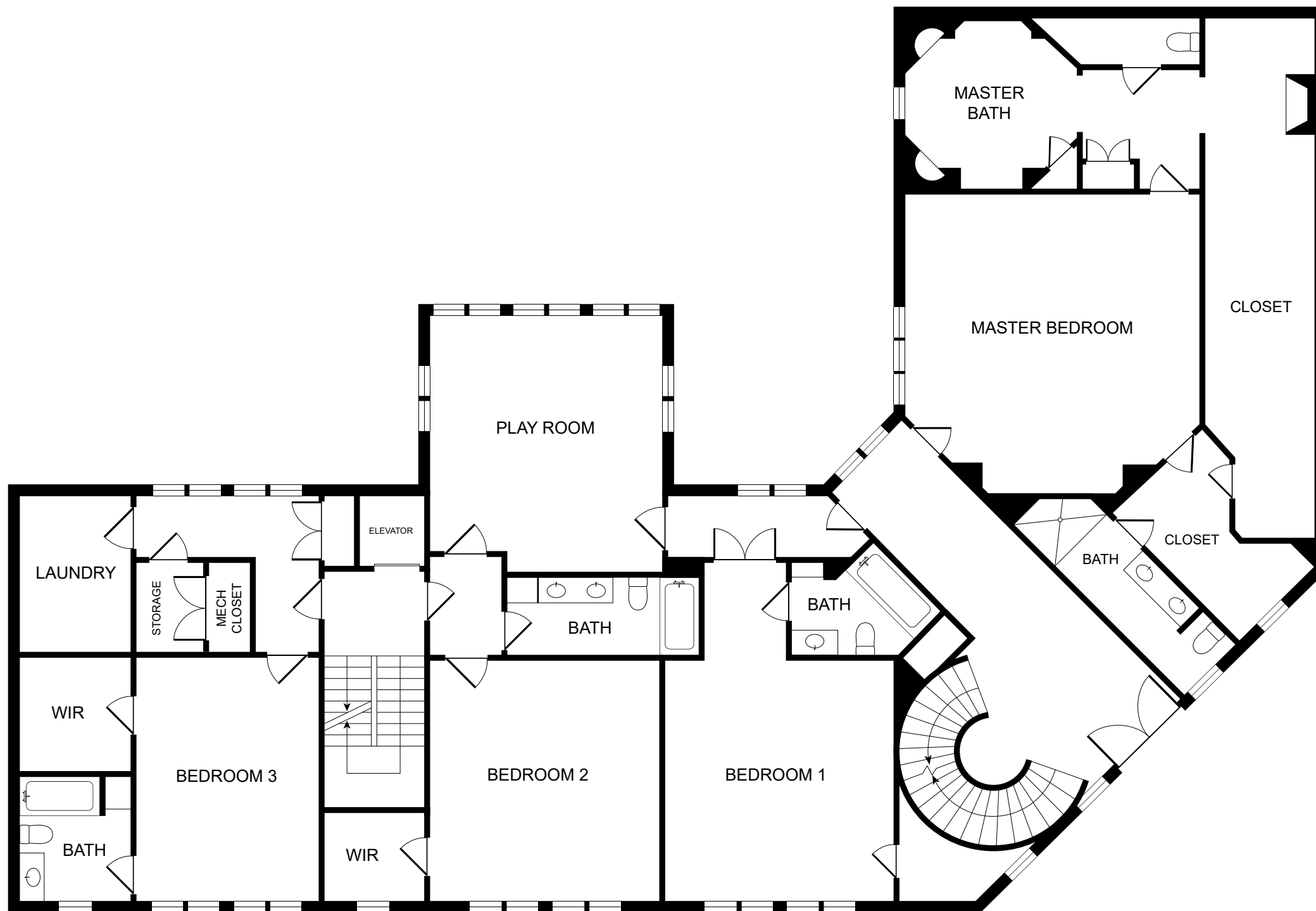
2ND FLOOR
