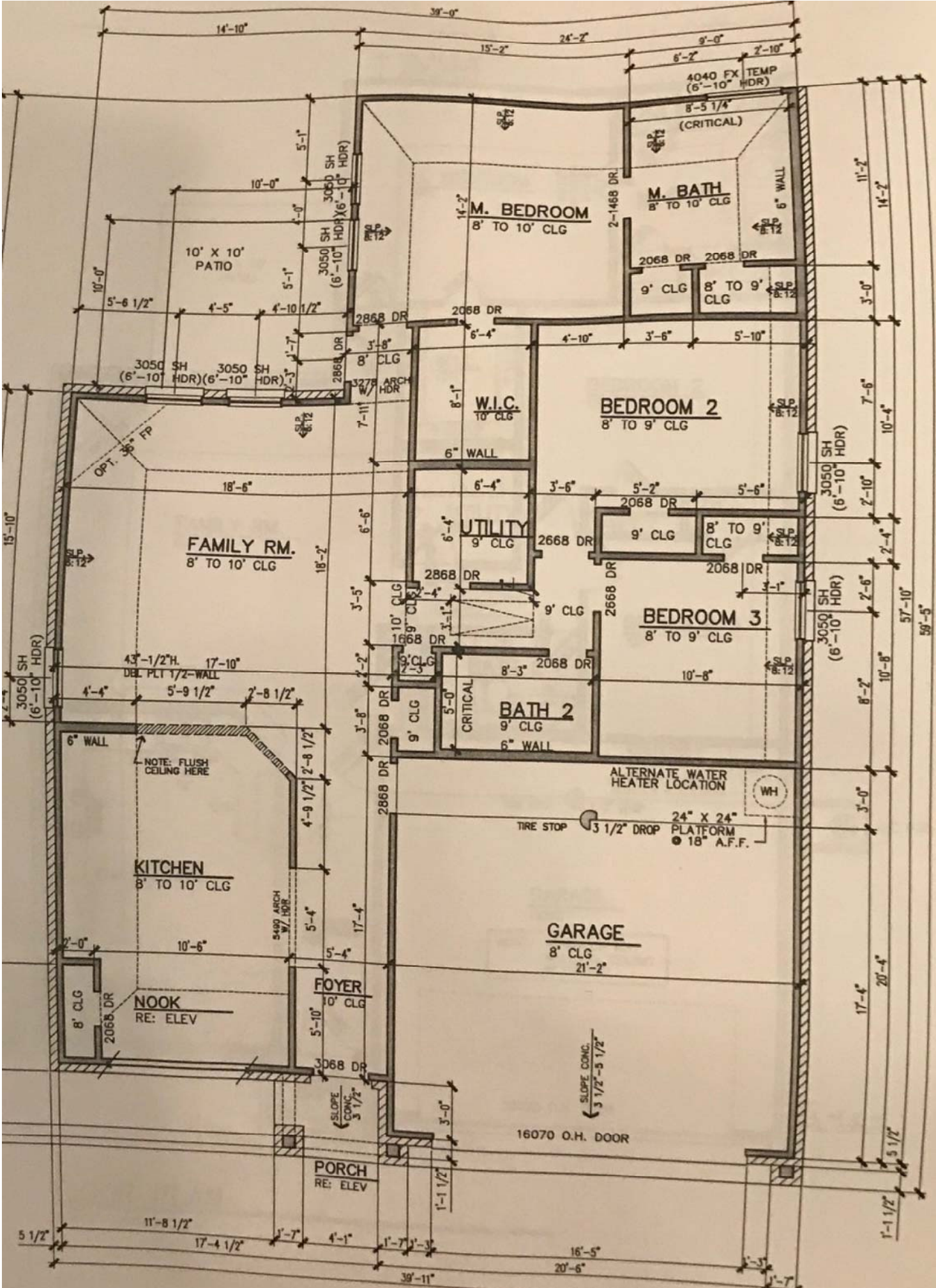
FLOOR PLAN
