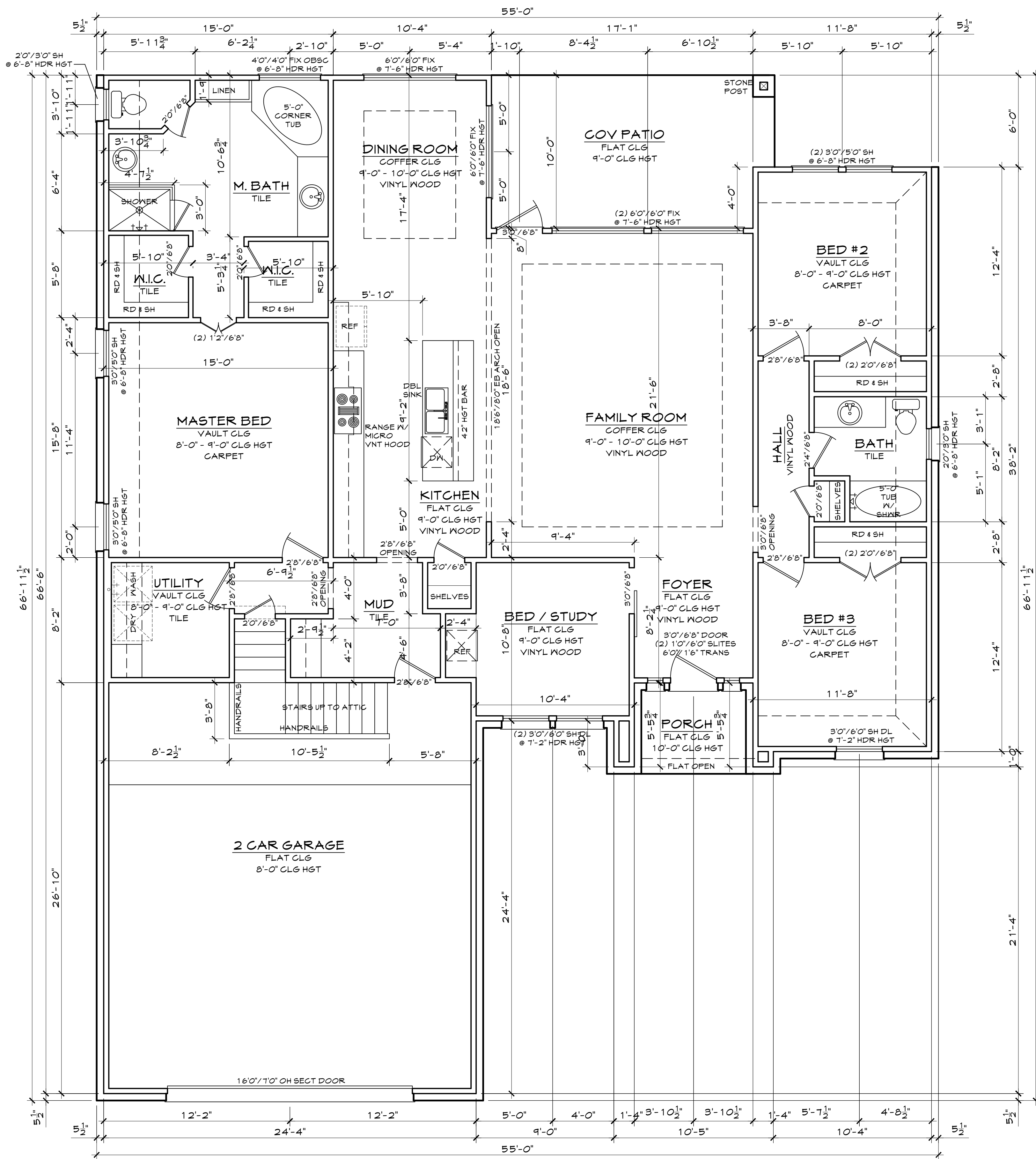
1 FLOOR PLAN A2 SCALE: 1/4" = 1'
