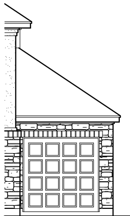
3499 ELEVATION "D" W/ 3RD CAR GARAGE
