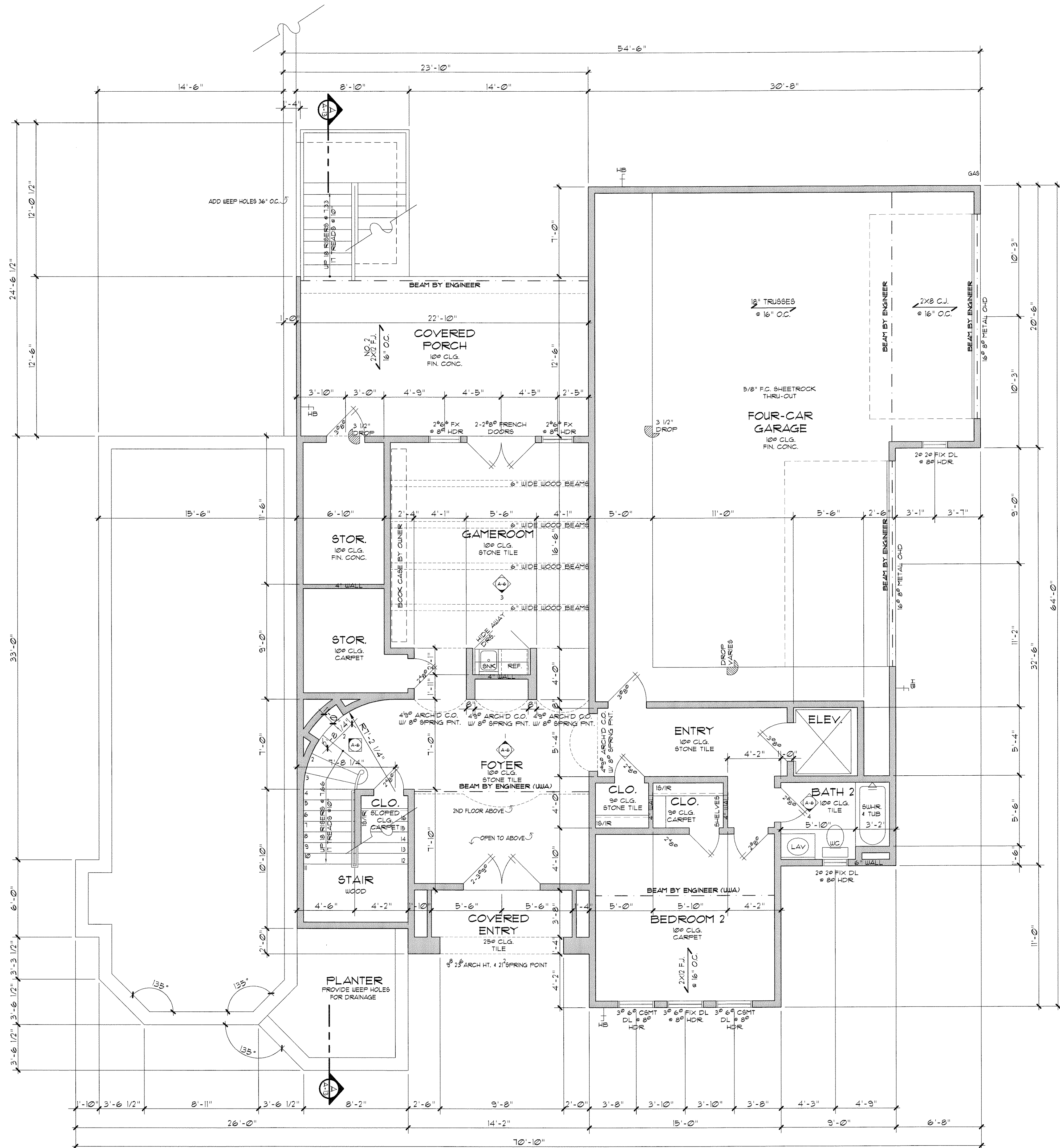
FIRST FLOOR PLAN SCALE: 1/4" = 1'-0"
