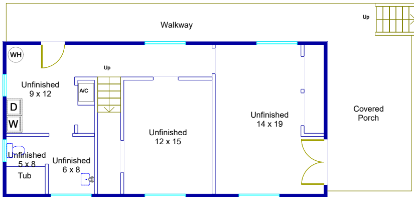
Guest House First Floor
