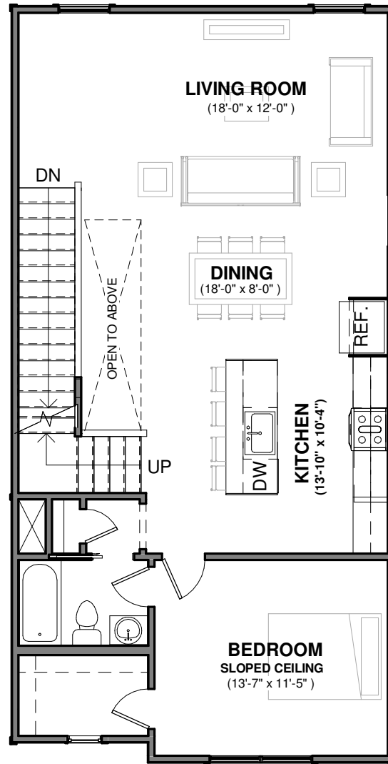
2/ Second Floor 1/8" = 1'-0"
