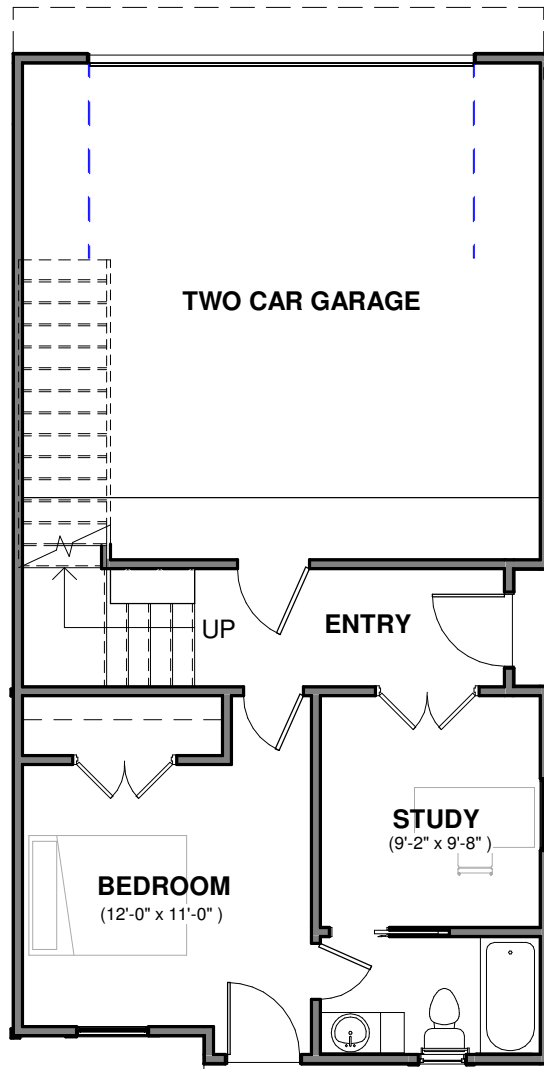
1/ First Floor 1/8" = 1'-0"
