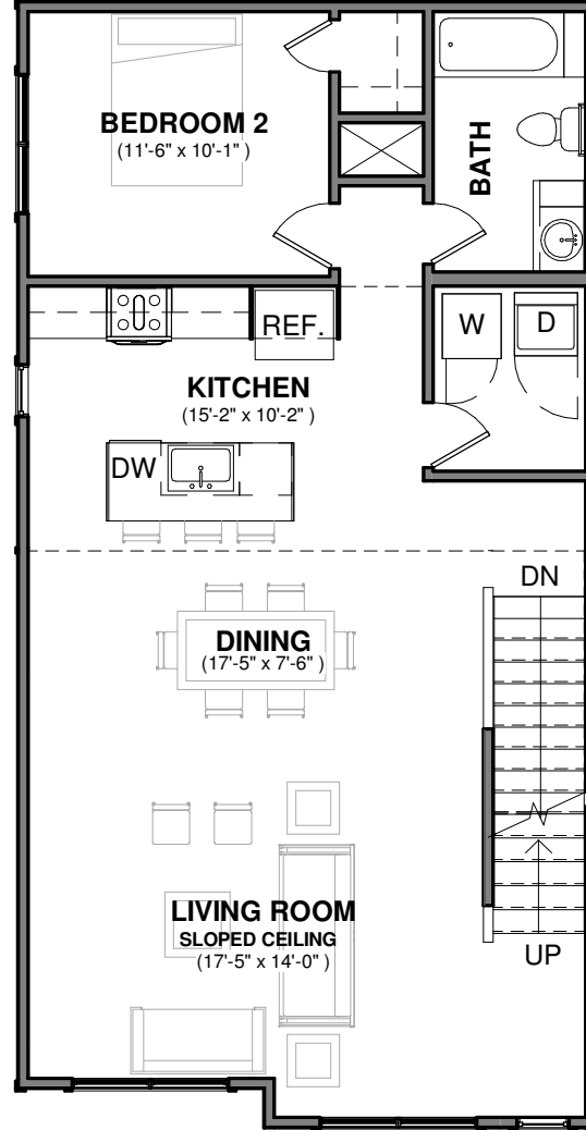
2/ Second Floor 1/8" = 1'-0"
