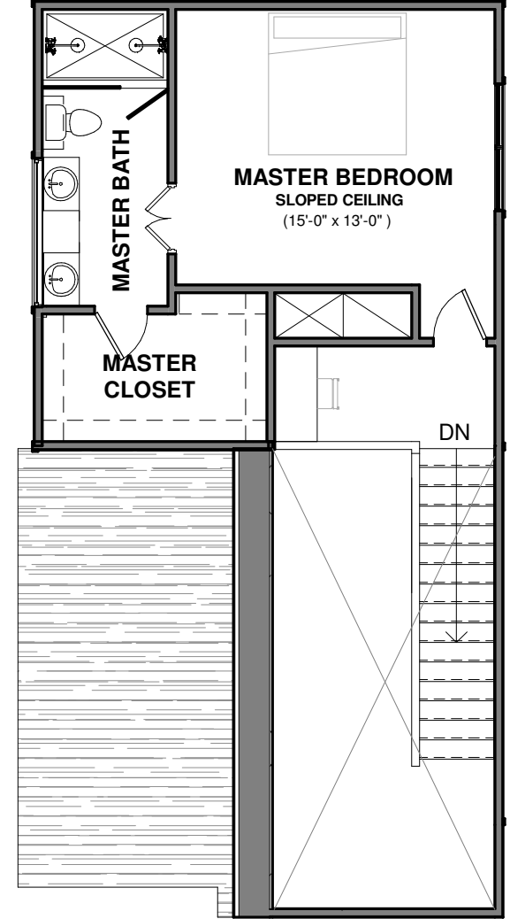
3/ Third Floor 1/8" = 1'-0"
