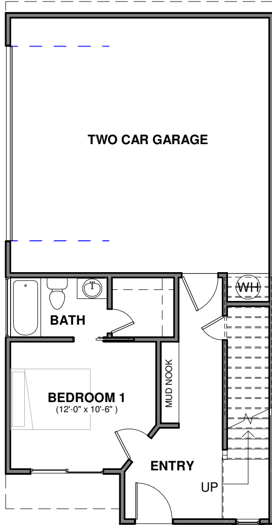
1/ First Floor 1/8" = 1'-0"
