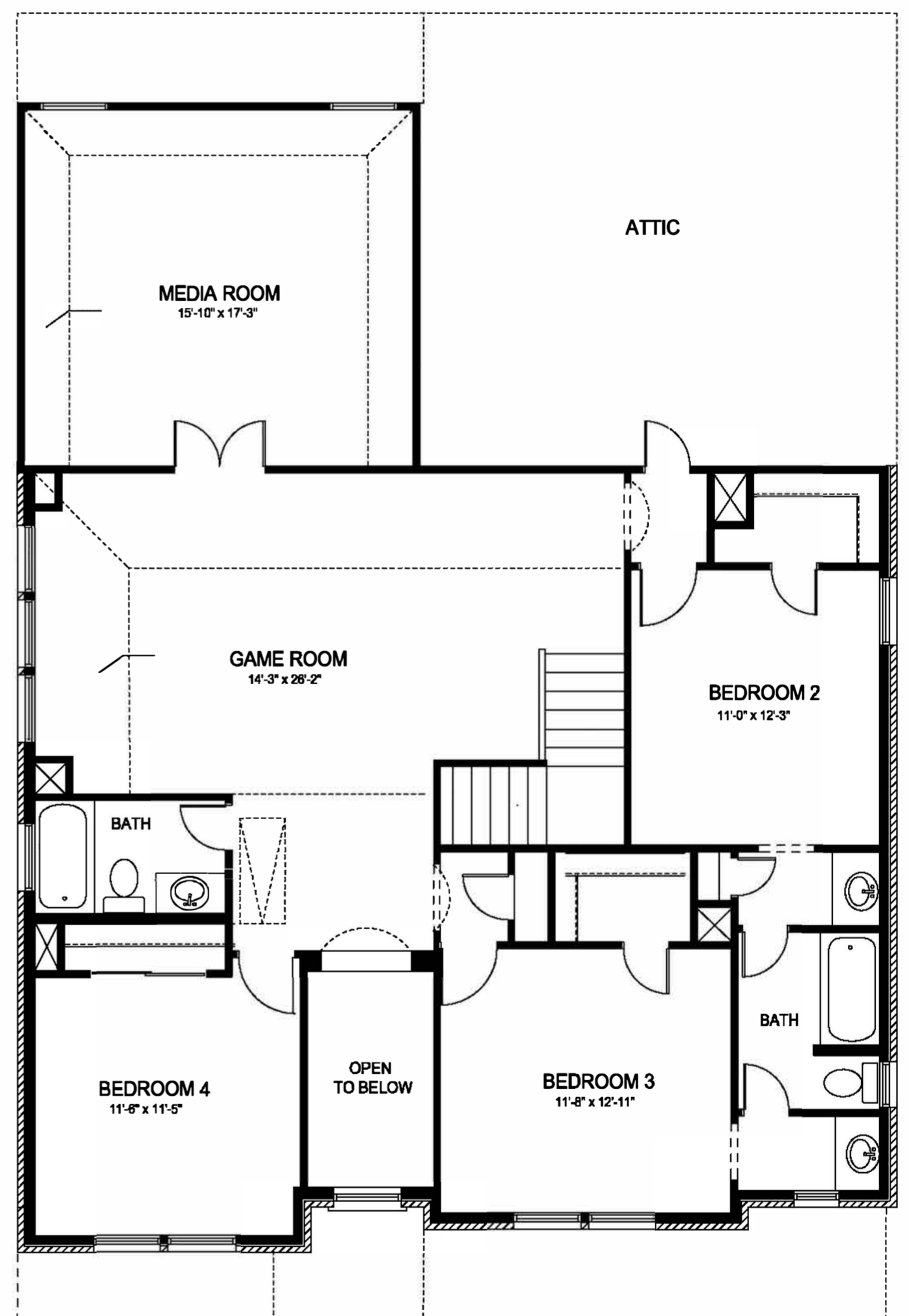
SECOND FLOOR
