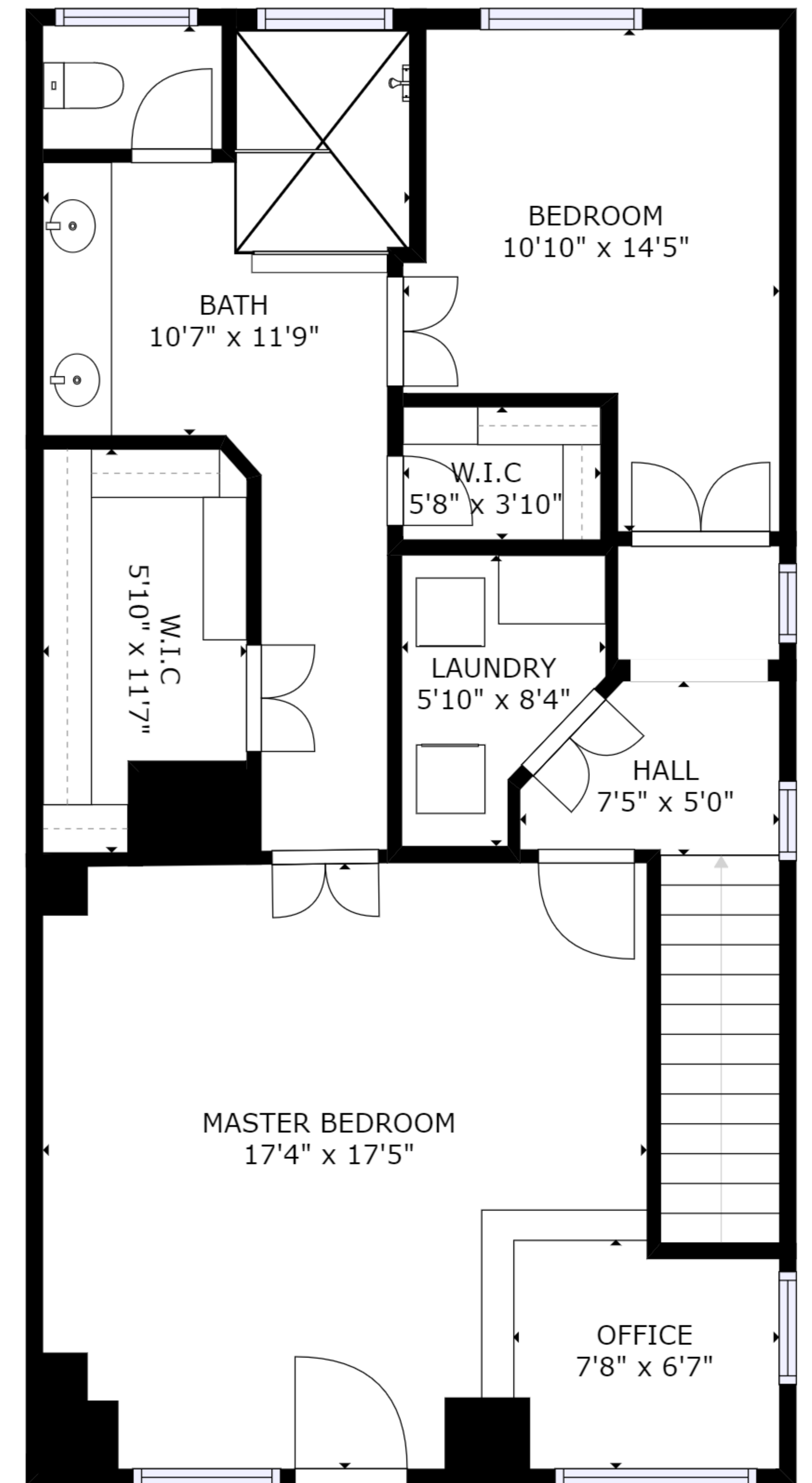
FLOOR 3
