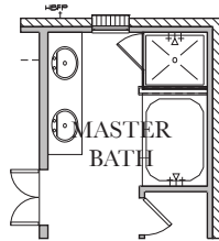
OPT. MASTER BATH TUB / SHOWER
