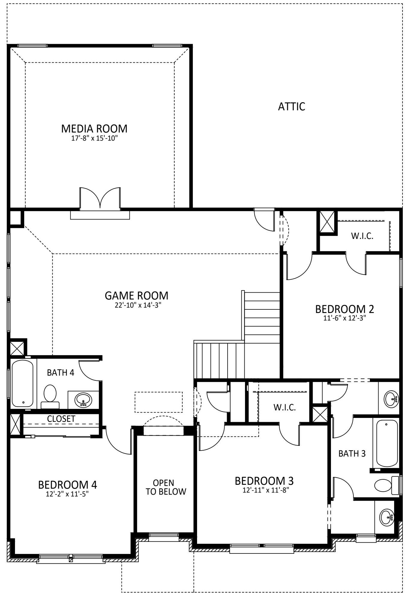
SECOND FLOOR
