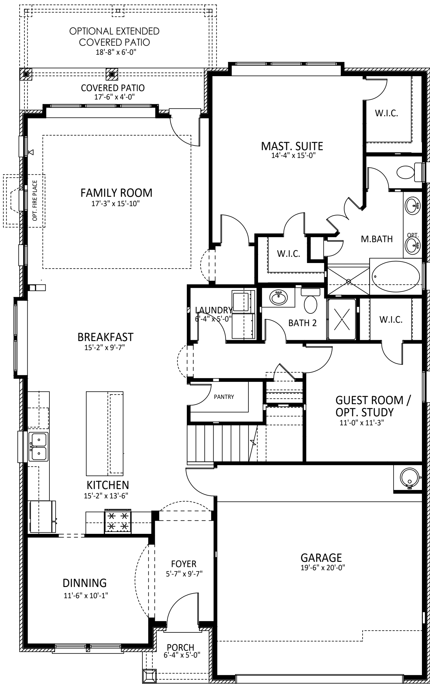
FIRST FLOOR
