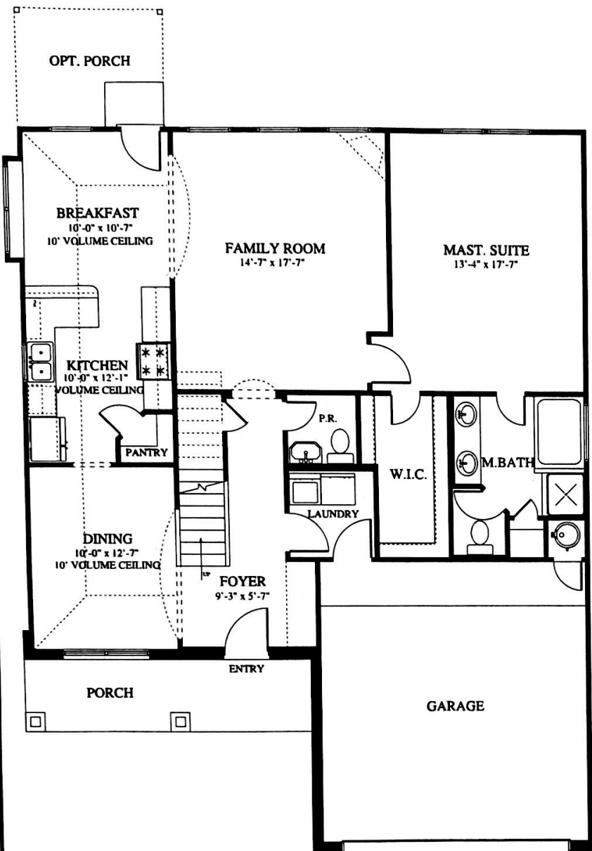
FIRST FLOOR PLAN 1282 S.F.
