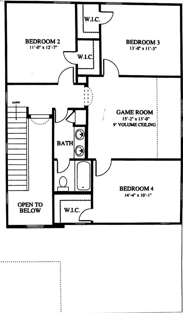
SECOND FLOOR PLAN 878 S.F.
