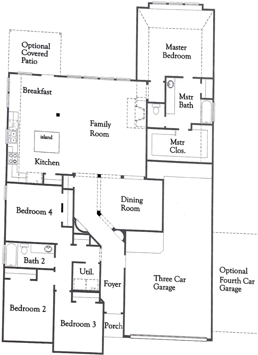
Floor Plan
