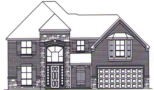
Elevation C
