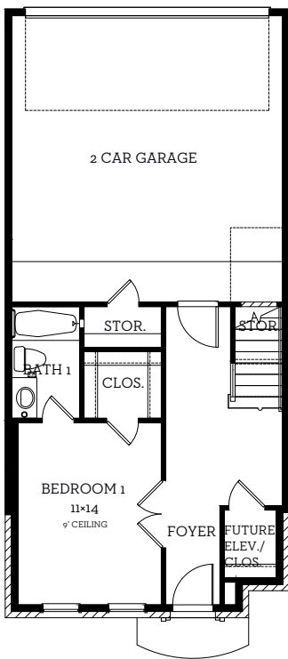
First Floor 464 sq.ft.
