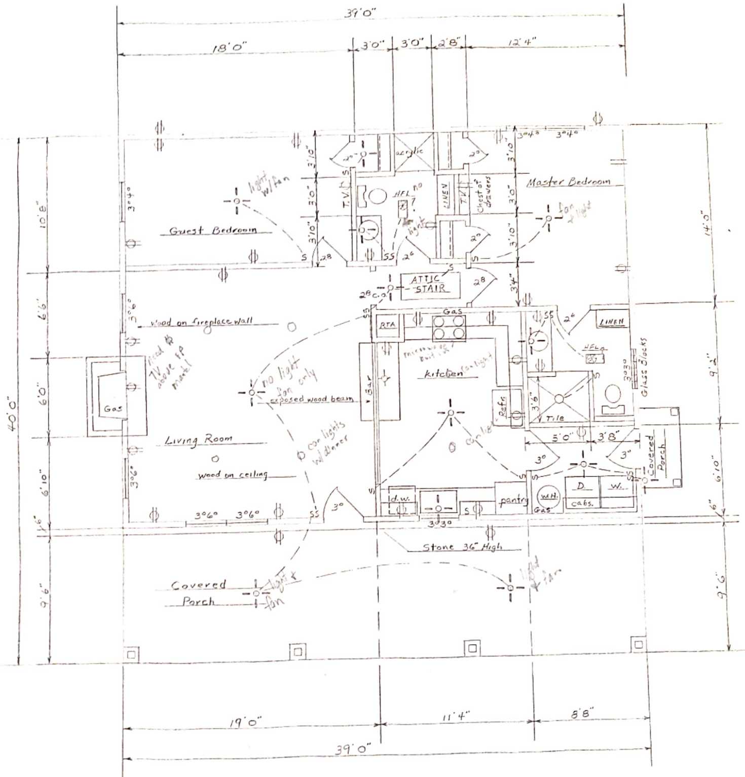
Floor Plan 1/4" = 1'
