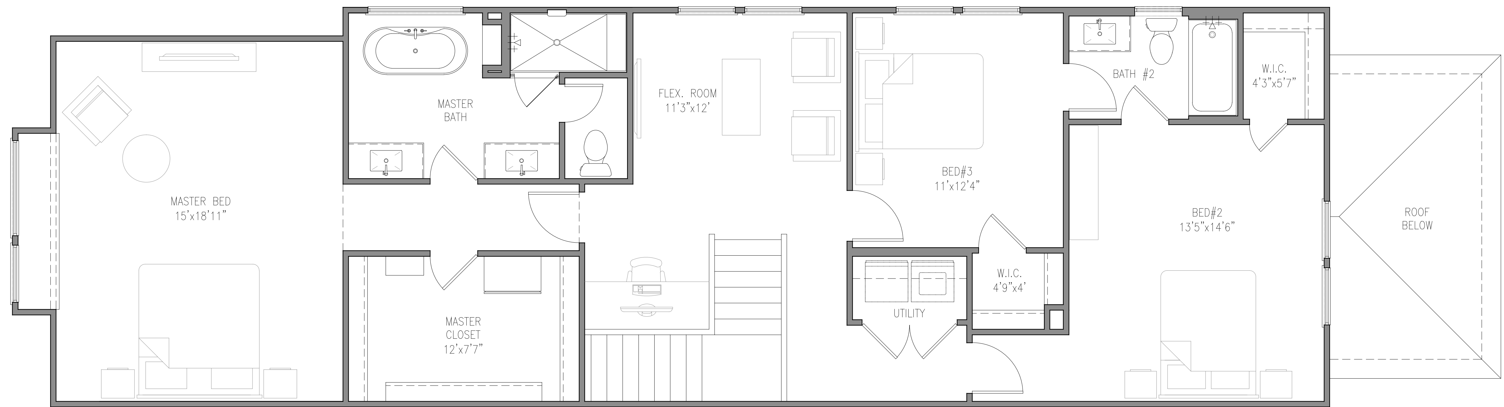
2ND FLOOR PLAN
