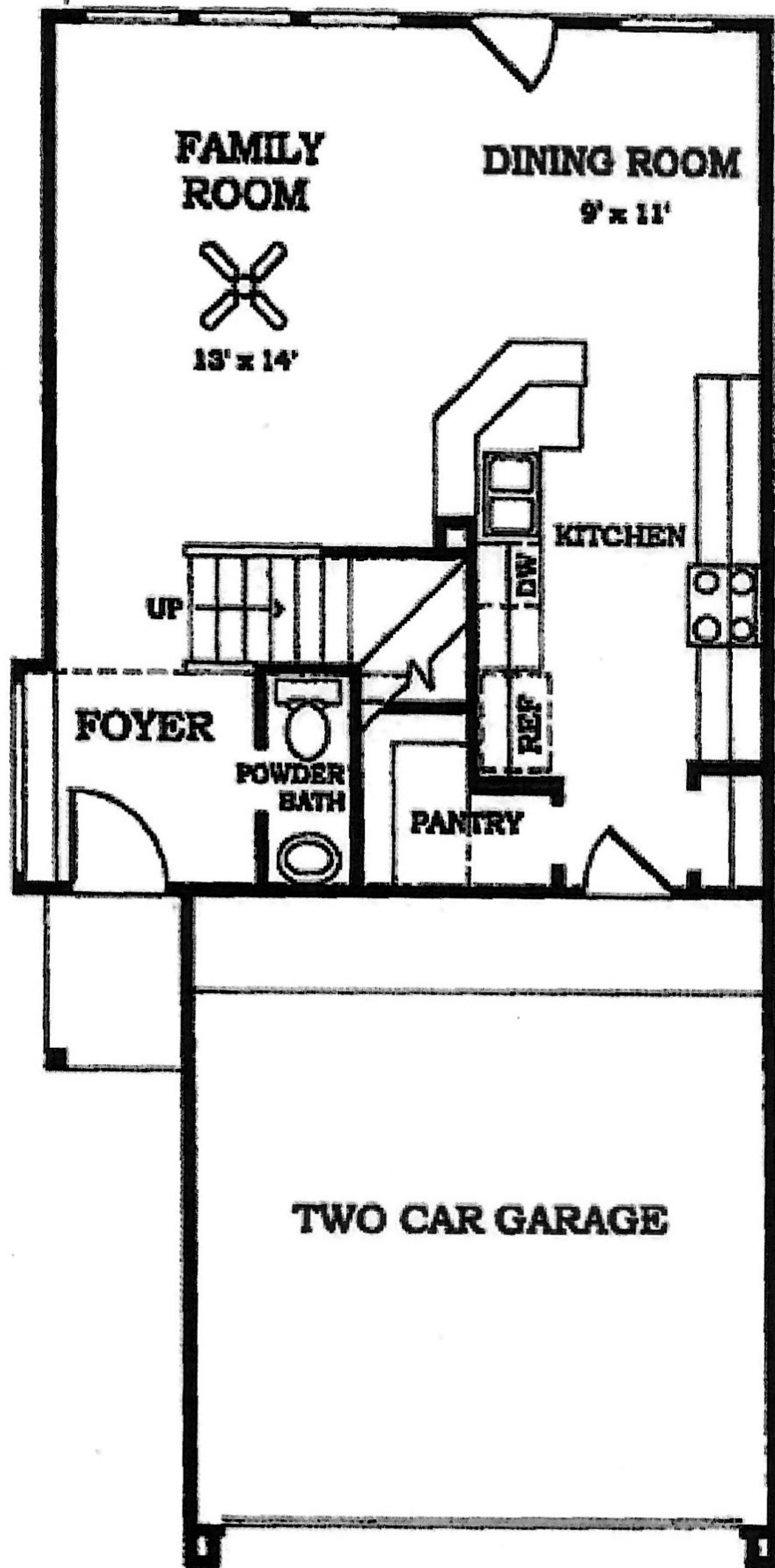
FIRST FLOOR
