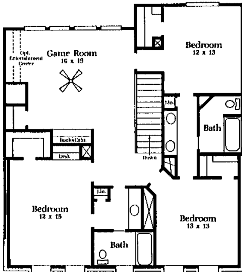
Second Floor
