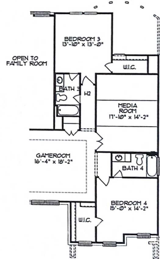
2ND FLOOR PLAN OPT. #0612 MEDIA ROOM FROM BEDROOM 5
