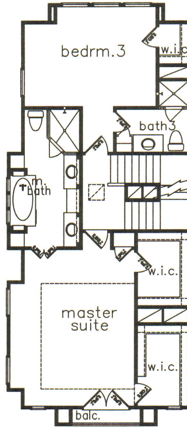
3RD FLOOR 978 SQ. FT.
