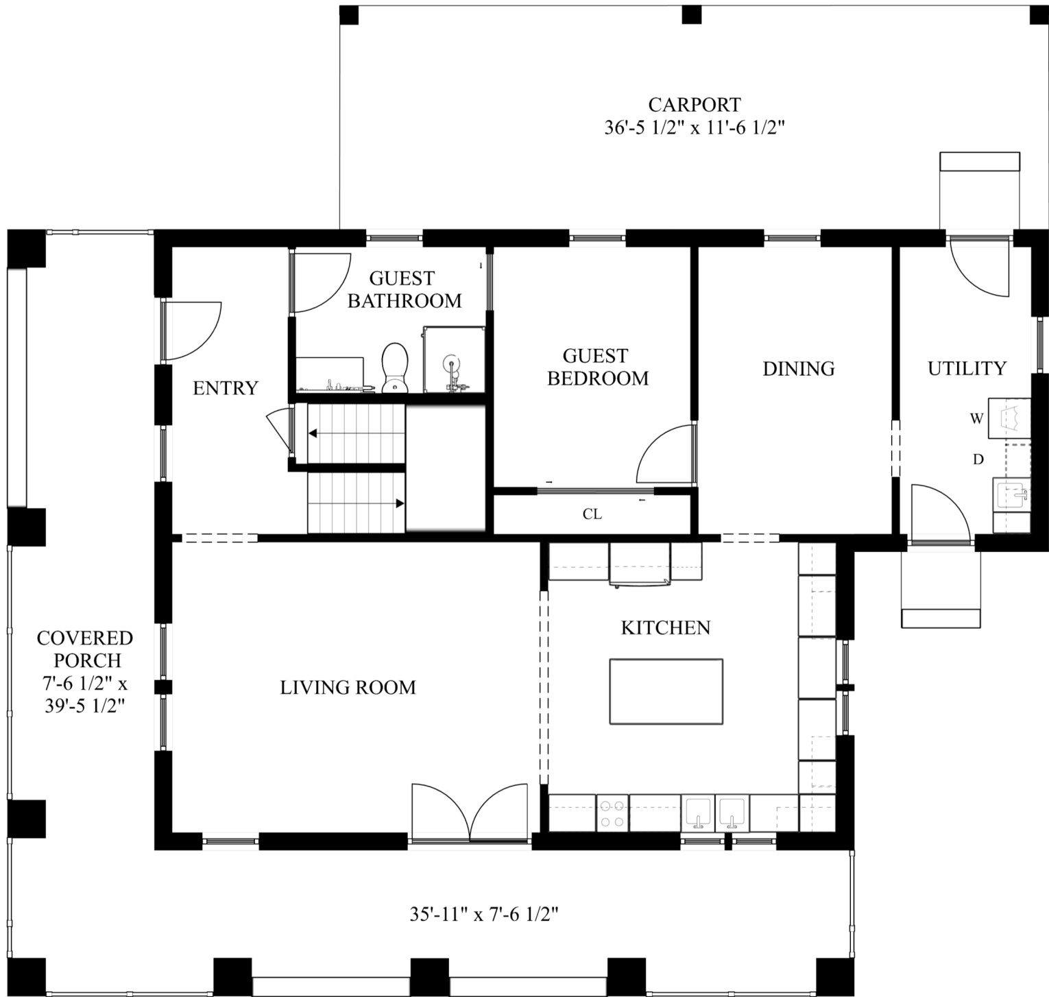
FIRST FLOOR
