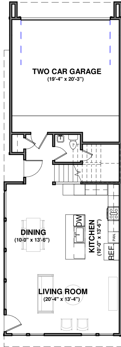
1/ First Floor 1" = 10'-0"
