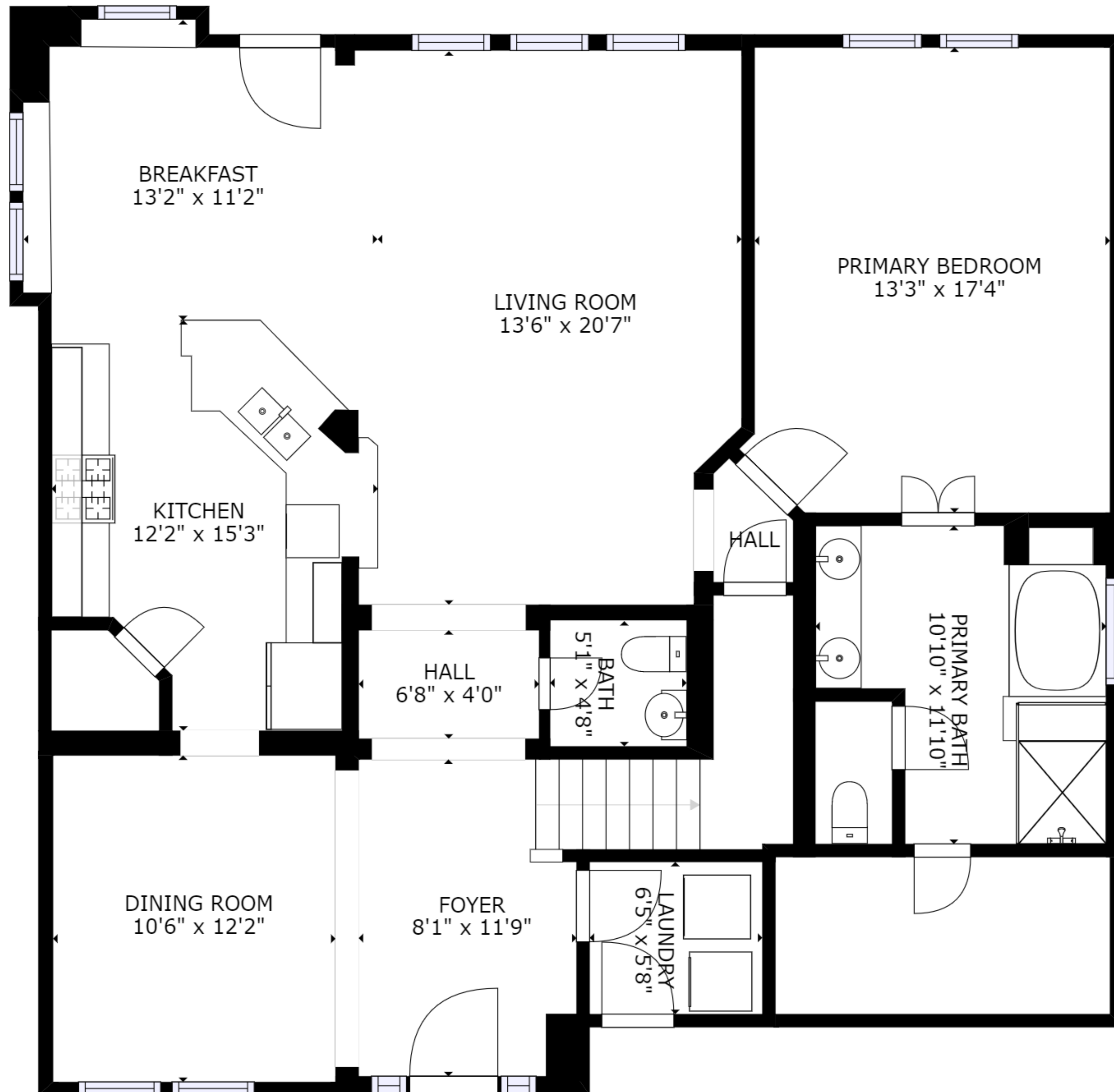
FLOOR 1
