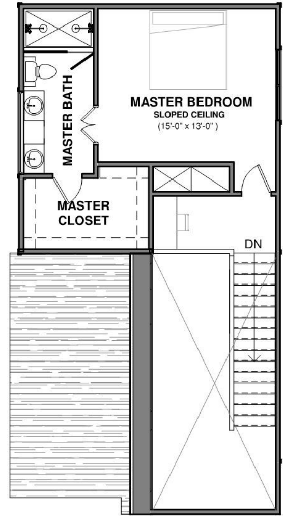
3/ Third Floor 1/8" = 1'-0"
