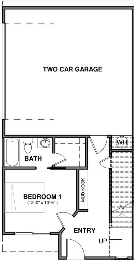
1/ First Floor 1/8" = 1'-0"
