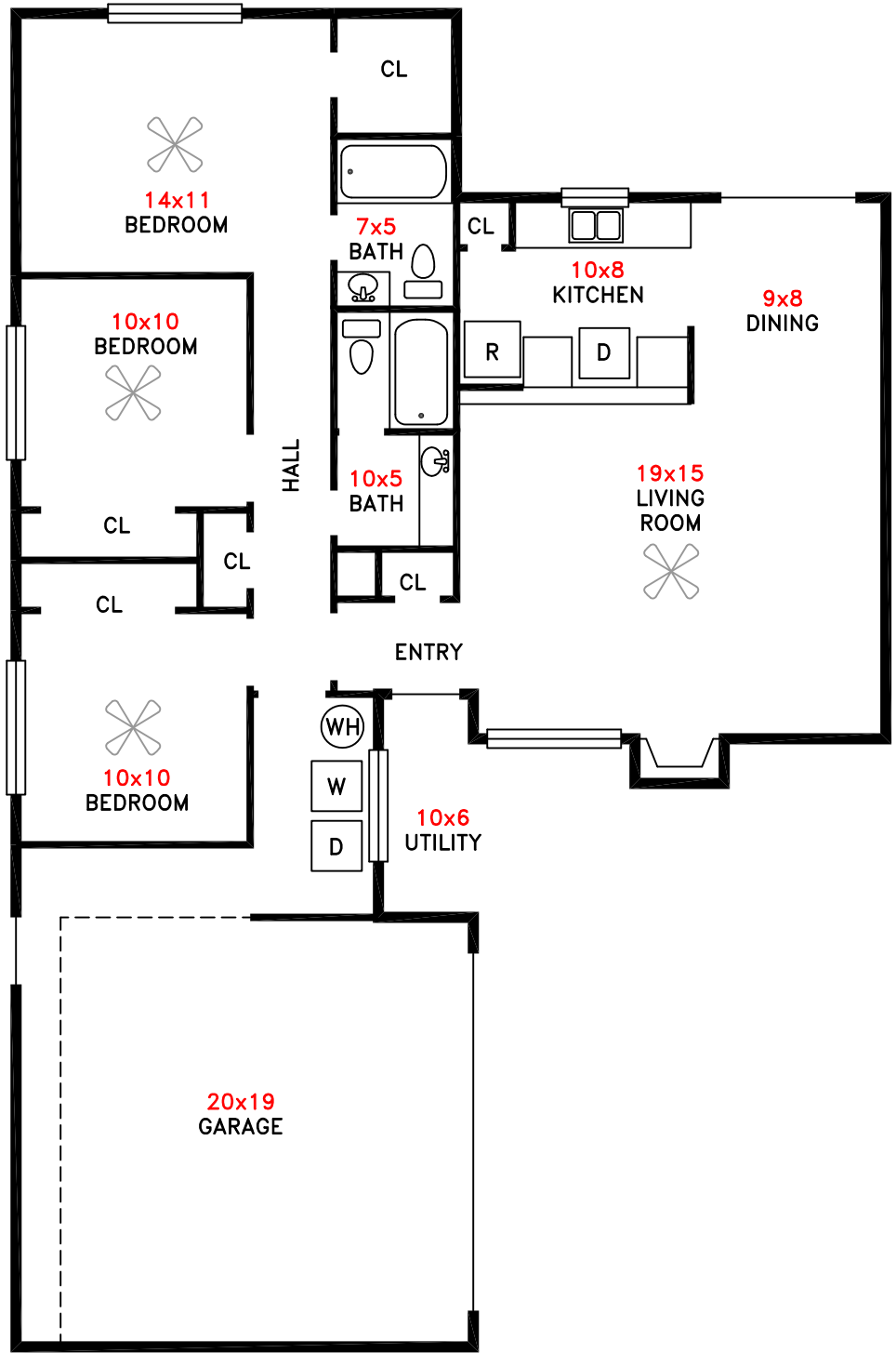
FLOOR-PLAN
