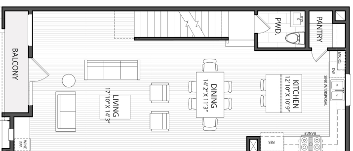
SECOND FLOOR 775 SQFT.
