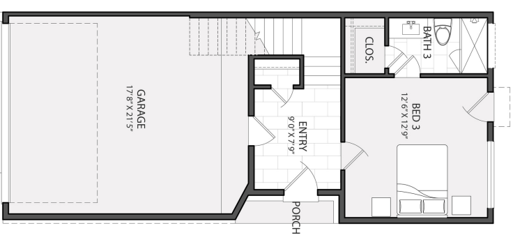
FIRST FLOOR 397 SQFT.
