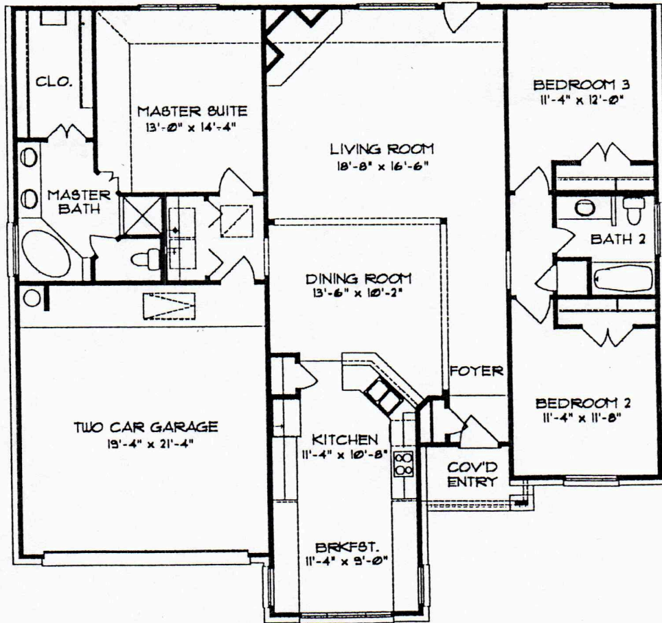
FLOOR PLAN
