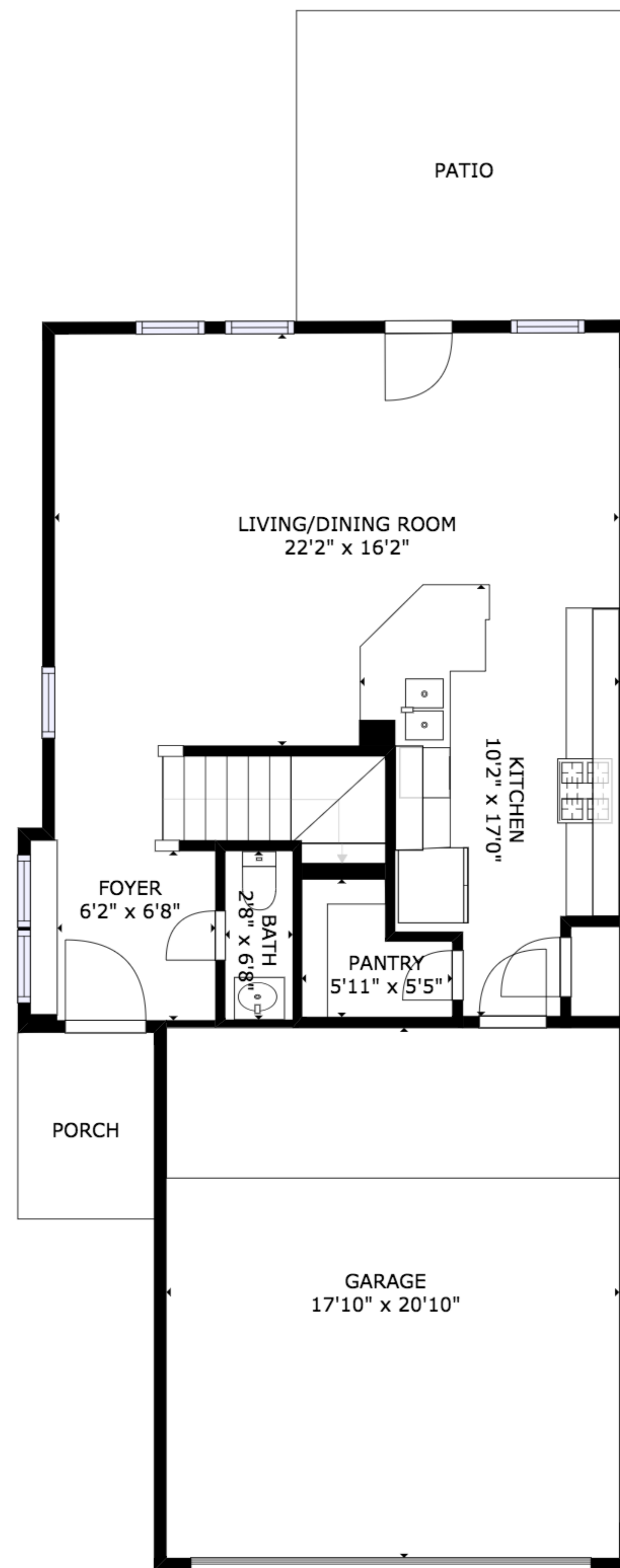
FLOOR 1
