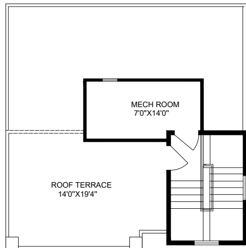
ROOF TERRACE
