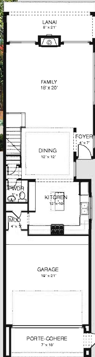
FIRST FLOOR
