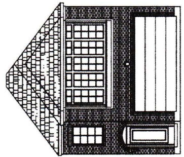
ELEVATION C
