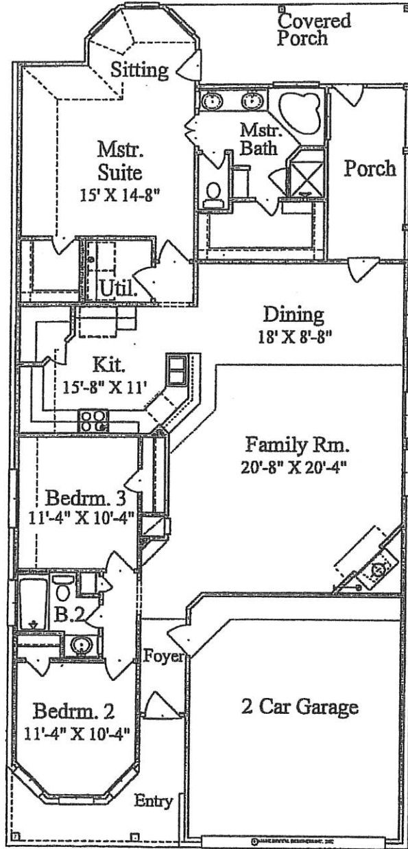
Floor Plan
