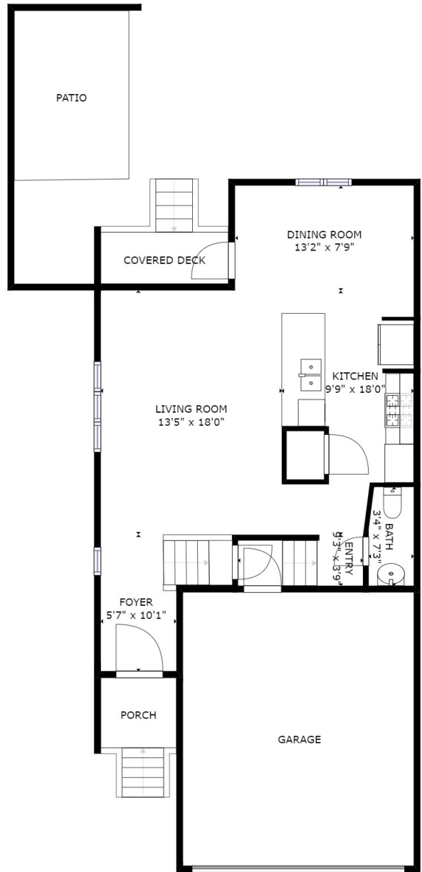
FLOOR 1
