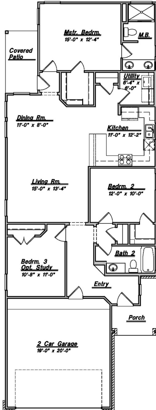
FLOOR PLAN Plan 1427
