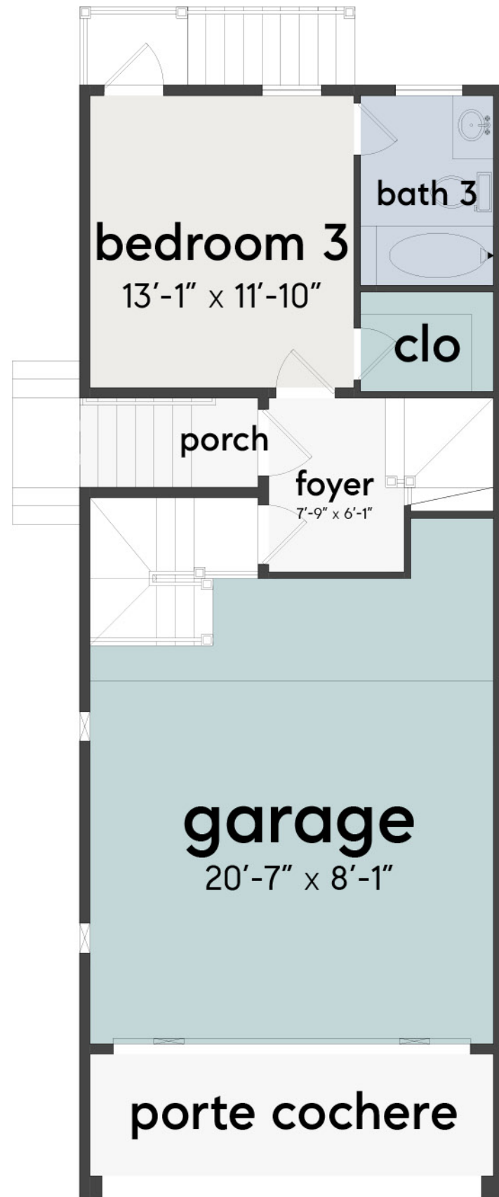
FIRST FLOOR
