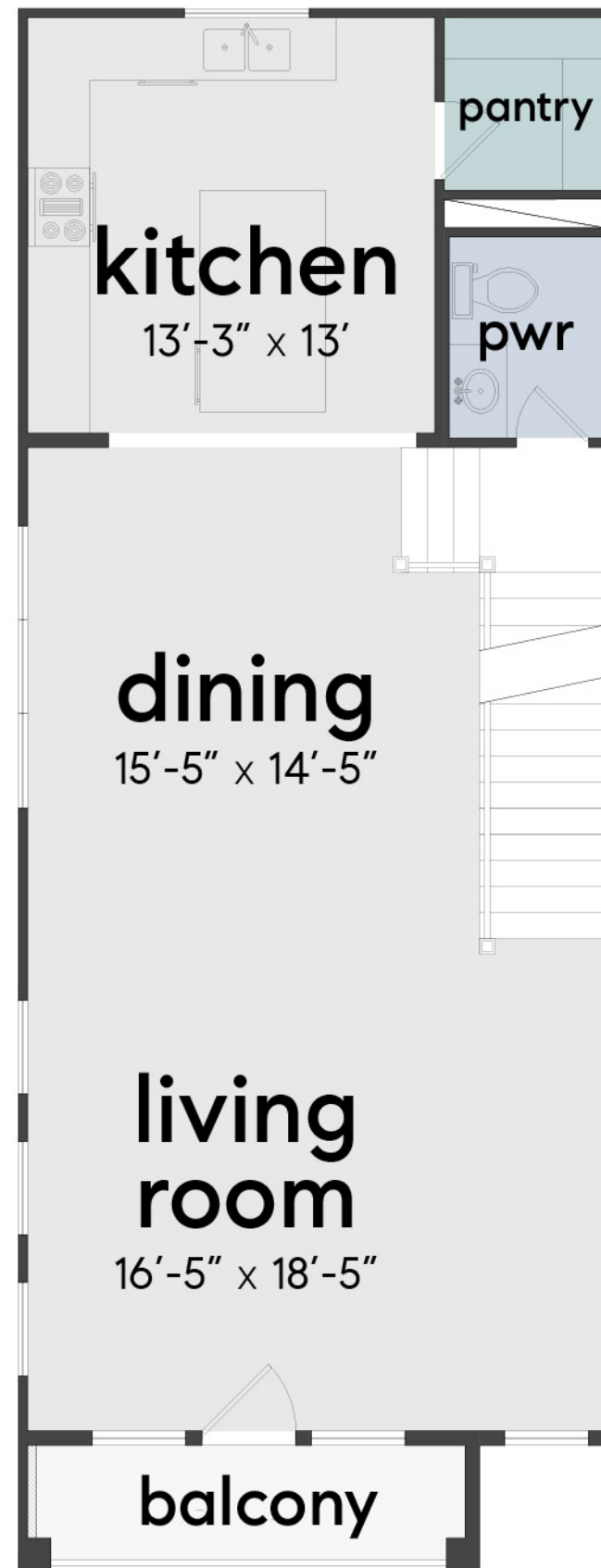
SECOND FLOOR
