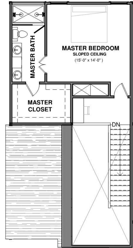
3/ Third Floor 1/8" = 1'-0"
