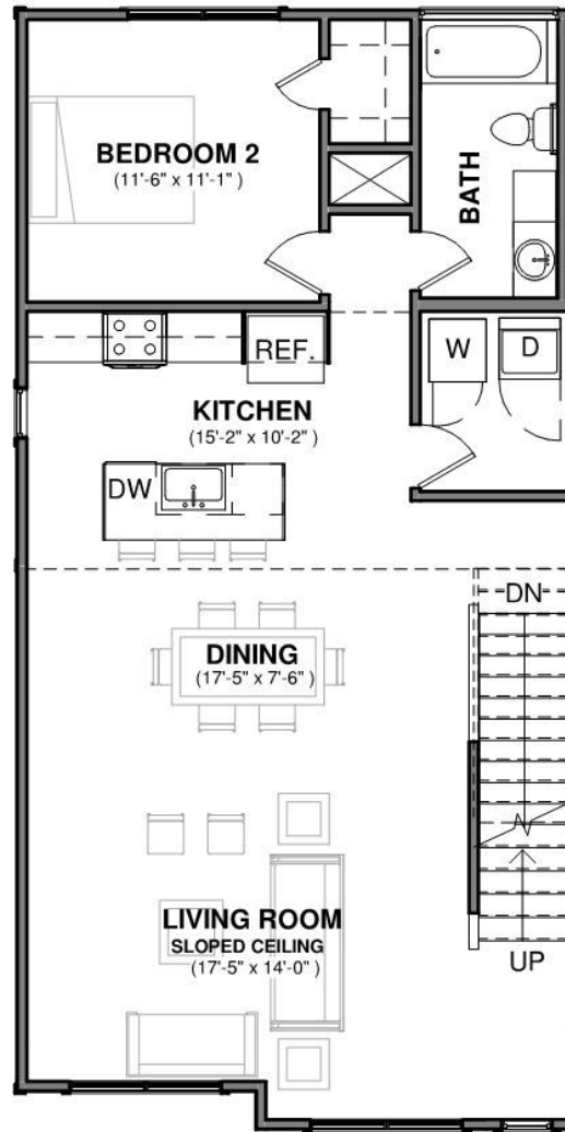
2/ Second Floor 1/8" = 1'-0"
